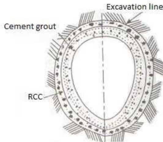
Figure 18.6 Egg-shaped Section
