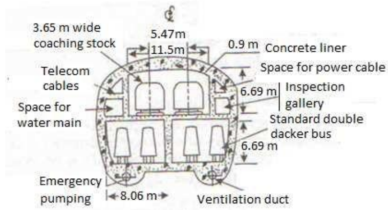
Figure Typical Cross-section of Multipurpose Tunnel
