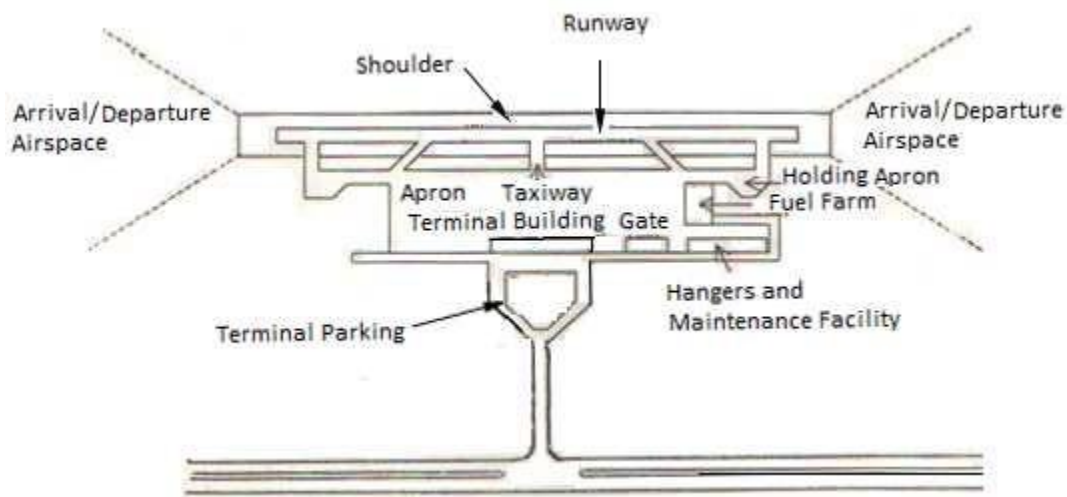
Figure 17.4 Typical Layout of Airport
