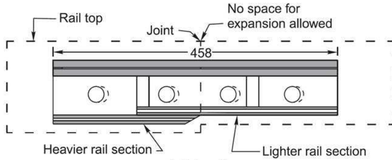
(b) Elevation
