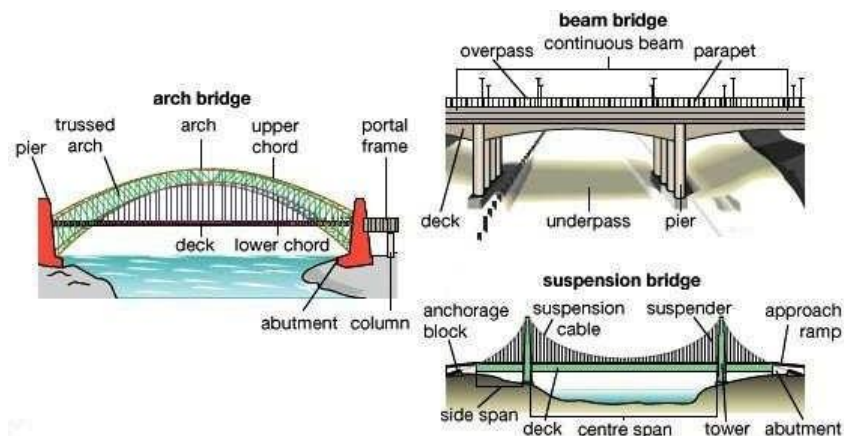
Types of Bridge
