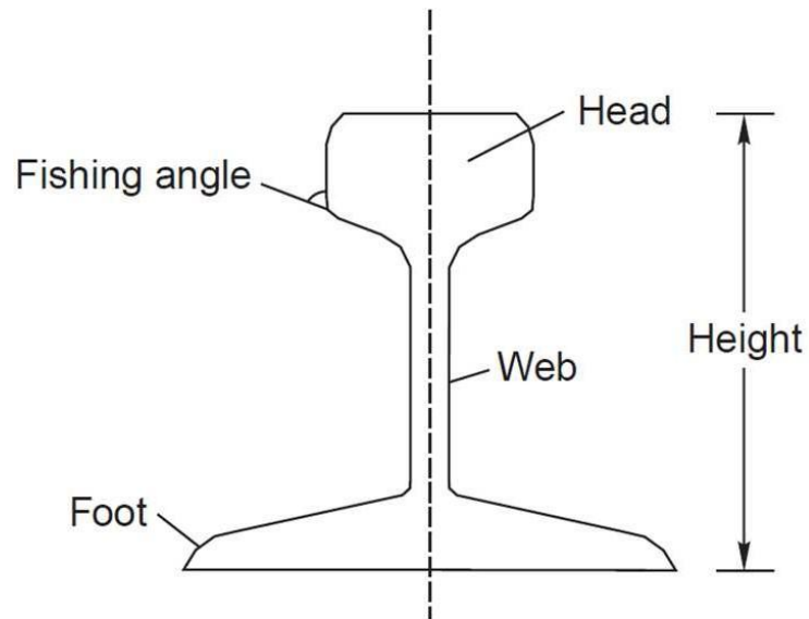
Flat-footed rail
