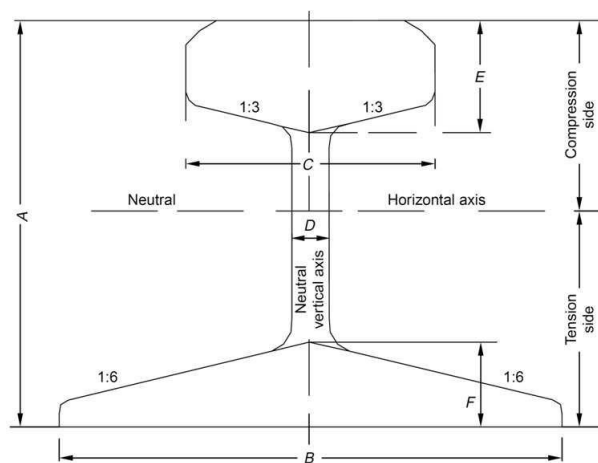
Standard flat-footed rail section
