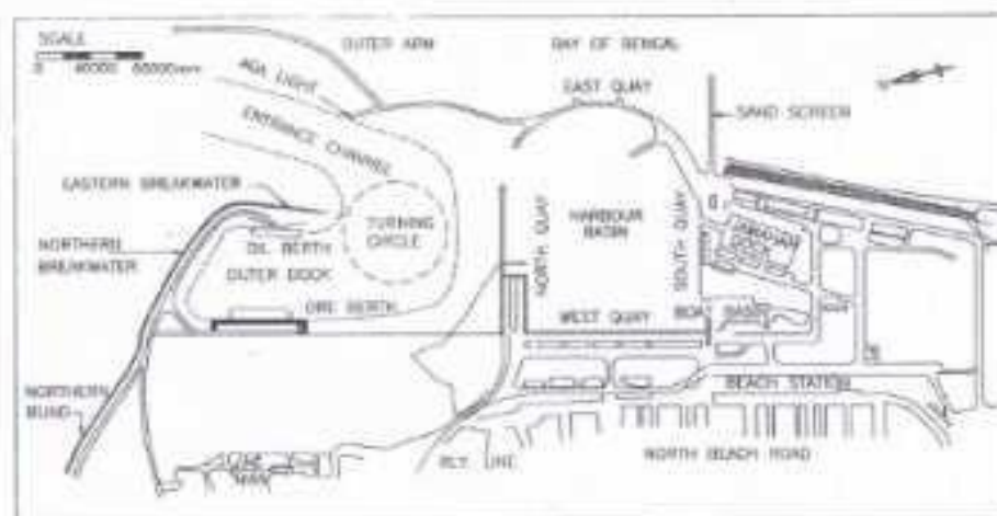
Fig. 13.1 Layout of Madras Harbour with outer Dock
