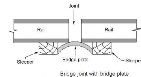
Bridge joint with bridge plate
