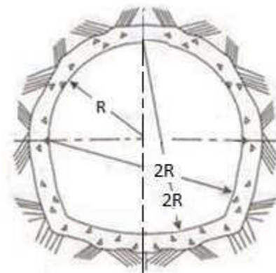
Figure 18.4 Horse-Shoe Section
