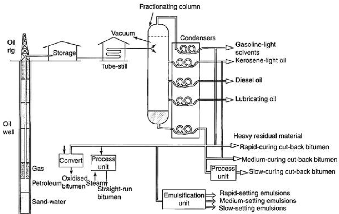
Fig. Schematic flow chat of petroleum refining
