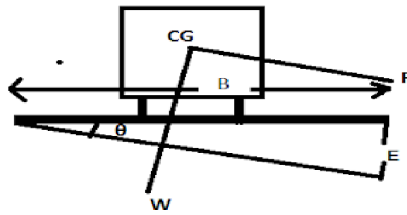
Super Elevation
