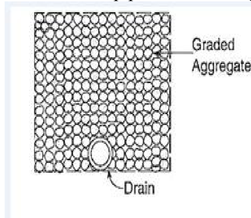
Fig. Geosynthetic-encased aggregate drain with a pipe
