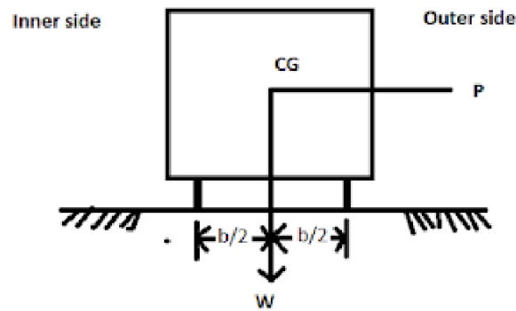
Overturning due to Centrifugal force
