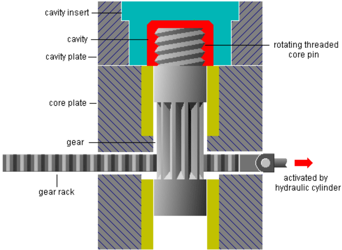
unscrewing device
