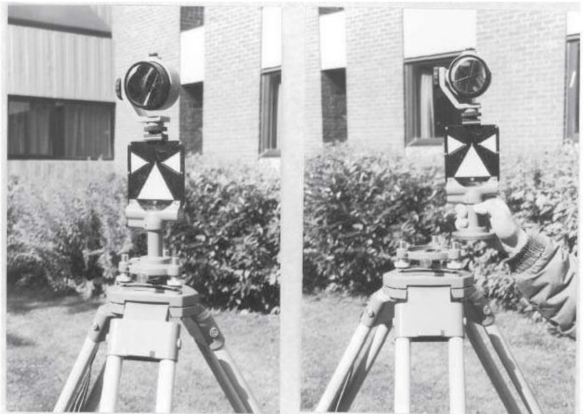
Figure 13.1. Interchangeable target and tribrach
